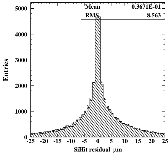
Fig. 13. Distribution of residuals for all hits ( \mu\text{m} ).
