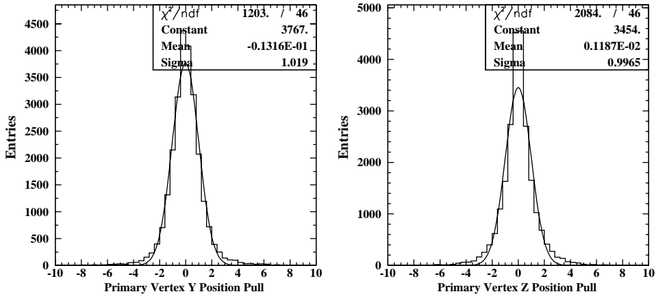
Fig. 19. Distributions of the pulls on y (left) and z (right) primary vertex position. The histograms are the data and the lines are Gaussian fits. The width of the Gaussians are very close to 1.0.
