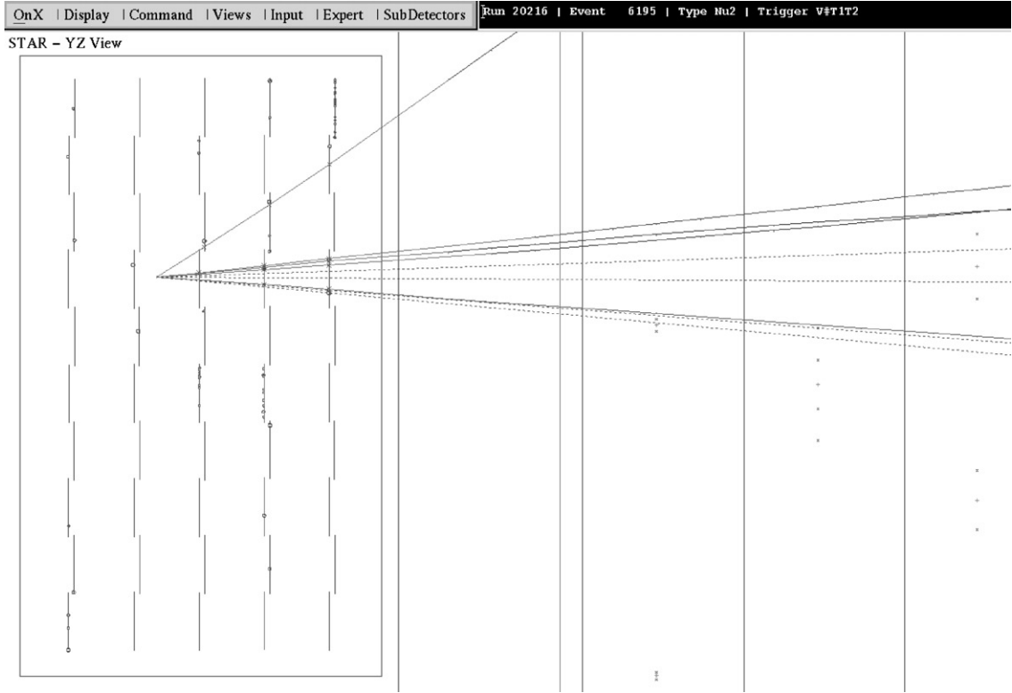
Fig. 20. Reconstructed \nu_\mu charged current event from the 1998 run.
