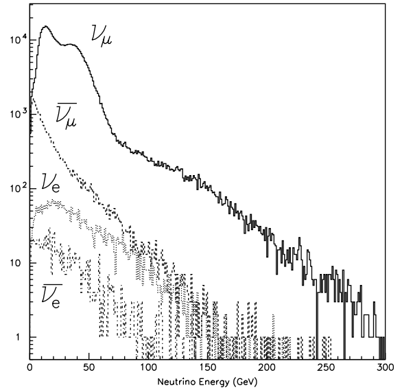
Fig. 4. The neutrino spectra of \nu_\mu , \bar{\nu}_\mu , \nu_e and \bar{\nu}_e at NOMAD-STAR as predicted by NUBEAM.
