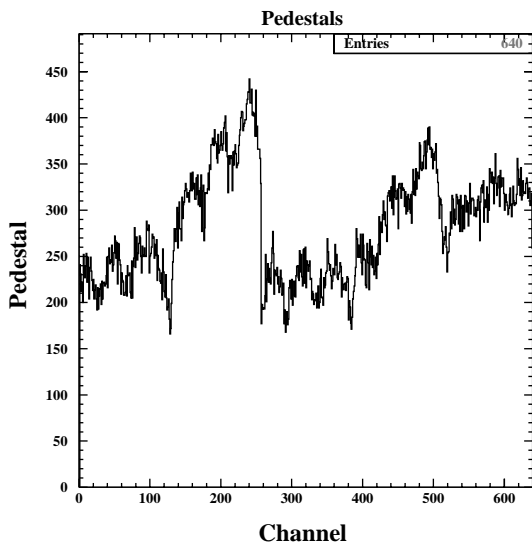
Fig. 5. The pedestals (in ADC counts) for the 640 channels of ladder 1 on layer 1. A channel-by-channel approach is used and the pedestals are recalculated for every run.
