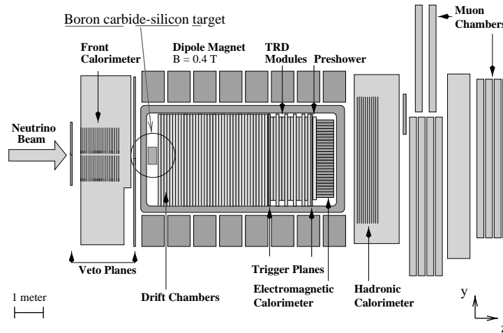
Fig. 2. The NOMAD detector with the Silicon TARget (NOMAD-STAR).
