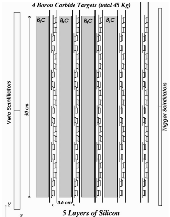
Fig. 3. Side view of the silicon target, showing the four boron carbide and five silicon layers (comprising 10 staggered ladders each), along with the veto and trigger scintillators. The neutrino beam enters from the left. Each silicon ladder is represented by the silicon sensor and the four carbon fibre rods that comprise the supporting backbone, all enclosed in the aluminium casing.
