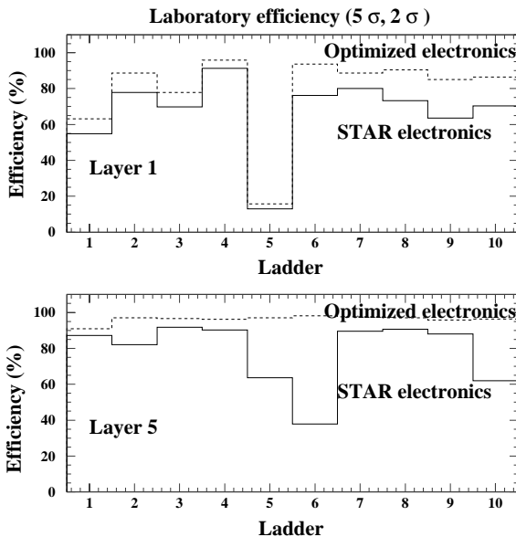
Fig. 12. Ladder efficiencies in the laboratory for layers 1 and 5.
