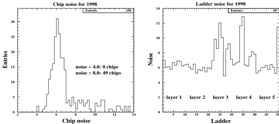
Fig. 8. (Left) The distribution of average chip noise for 1998; (right) the average noise for 1998 shown ladder-by-ladder.
