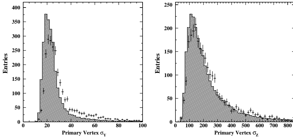
Fig. 17. Distributions of the reconstructed uncertainties in the y (left) and z (right) position of the primary vertex (in \mu\text{m} ).
