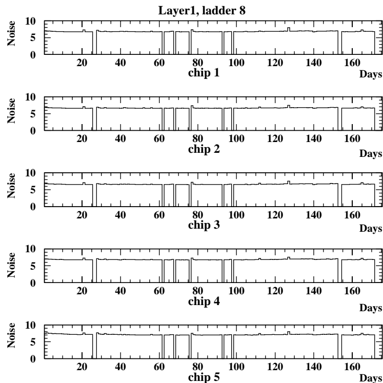
Fig. 6. Chip noise evolution in time. The horizontal axis represents the days in the 1998 run from April to September 1998. The vertical axis shows the RMS ADC noise count for the chip. The gaps correspond to days with no data.
