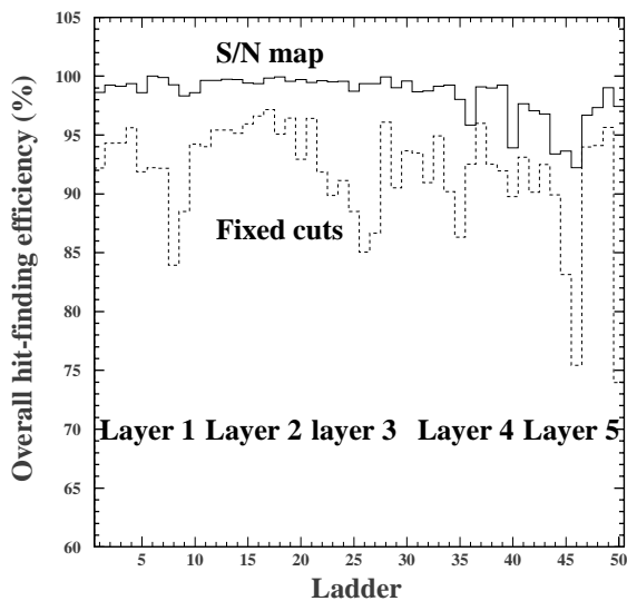
Fig. 10. The overall hit-finding efficiency by ladder for optimised and fixed S/N cuts. The solid line corresponds to the optimised cuts and the dashed line to fixed cuts.
