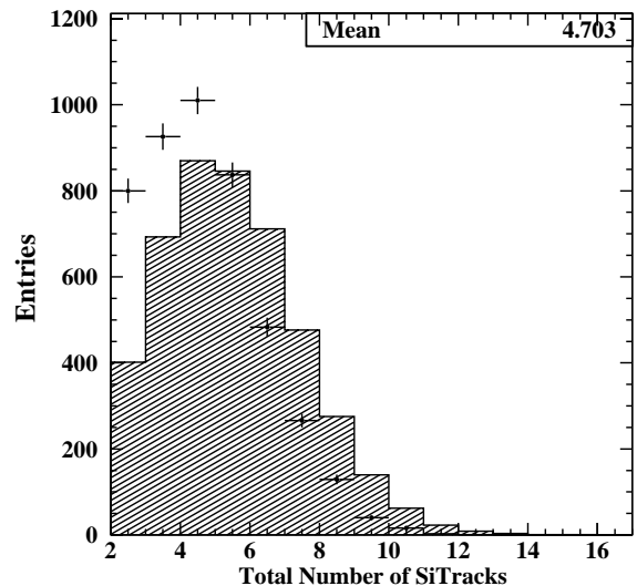
Fig. 14. Distribution of the number of NOMAD-STAR tracks in the primary vertex for data (points) and for \nu_\mu CC Monte Carlo (histogram). Note the excess of events with two or three tracks in the data due to the absence of quasi-elastic and resonance events in the simulation. The mean number of tracks per event found in the data is 4.7.
