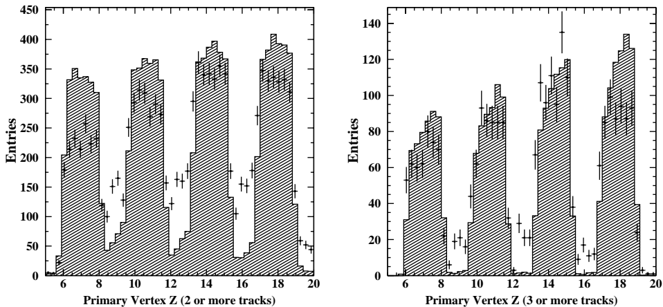
Fig. 16. Distributions of the z position of primary vertex (cm): (left) only two or more tracks in the vertex and (right) three or more tracks in the vertex.
