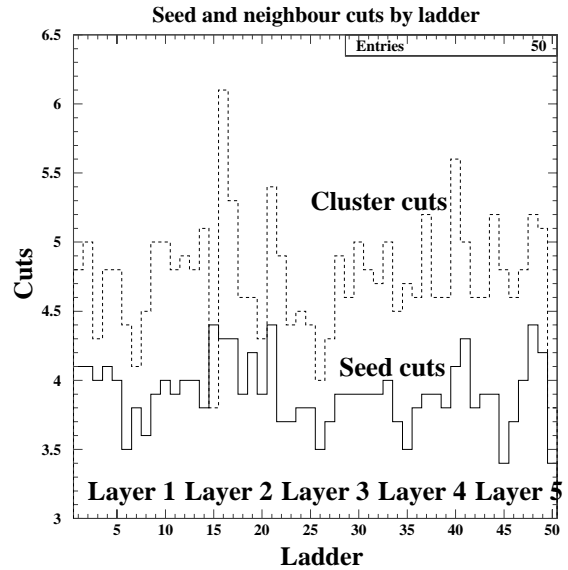
Fig. 9. The seed and cluster cuts by ladder. The solid line corresponds to the seed cut and the dashed line to the cluster cut.
