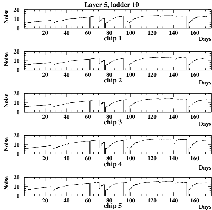
Fig. 7. Noise evolution for unstable chips for April through to September 1998. The vertical axis shows the RMS ADC noise count for the chip. The gaps correspond to days with no data.
