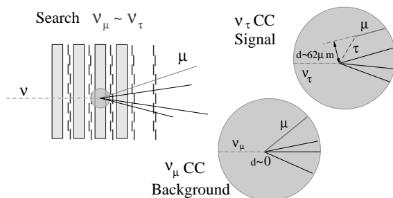
Fig. 1. Definition of the impact parameter.
