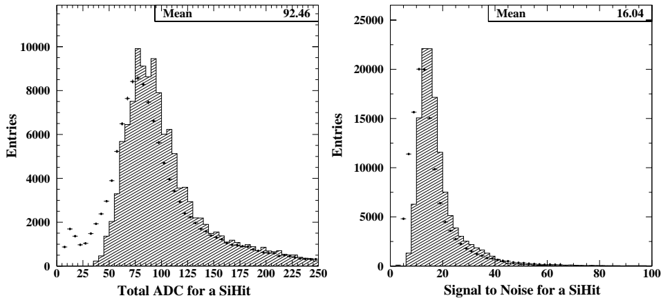
Fig. 11. (Left) Total ADC signal selected in a cluster by the S/N cuts; (right) total signal to noise distribution in a cluster selected by the S/N cuts. The data points are overlaid on the \nu_\mu CC Monte Carlo histogram, which has been normalised to the data. The mean values correspond to the data.
