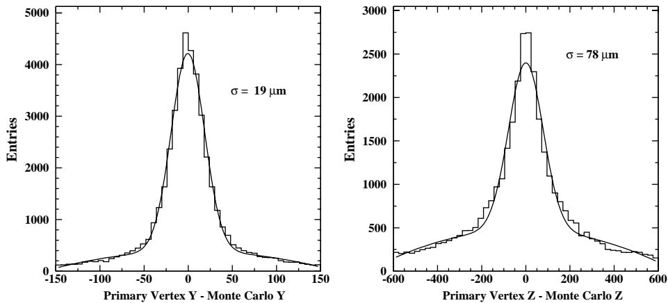
Fig. 18. Distributions of the y (left) and z (right) position accuracy of the reconstructed primary vertex (in \mu\text{m} ). The histograms are the data and the lines are fits to double Gaussians. The width of the central Gaussian is also shown.
