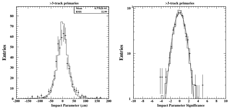
Fig. 21. Impact parameter distribution (left) and impact parameter significance (right) of \nu_\mu CC data (points) and Monte Carlo (histogram) for all events with three or more tracks in the hadronic vertex.
