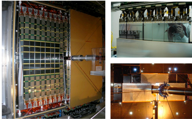
Figure 1: View of the TT installed in LHCb (left). View of the first IT station (bottom right), and detail of one of the detector boxes (top right).
