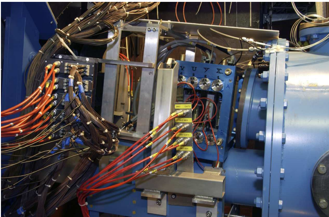
Figure 2.4: Photography of the three detectors installed upstream the magnet, between the first vacuum chamber (right-hand side) and the secondary particle channel. From right to left, the GEM/MSGC, SFD and IH detectors can be found. The primary proton beam line can be appreciated at the bottom.
