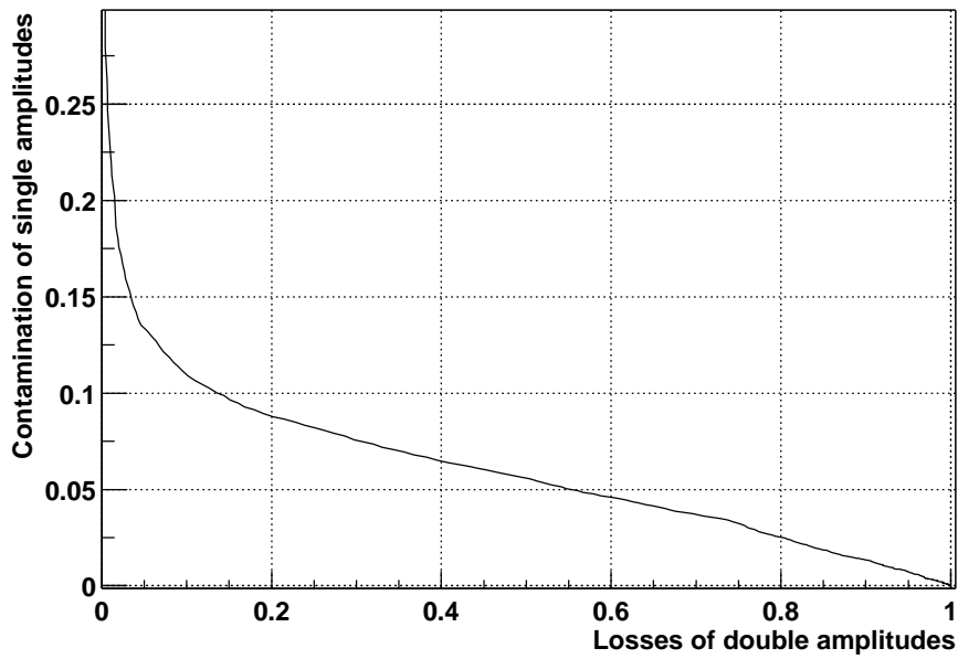
Figure 2.10: Contamination of single ionization amplitudes as a function of losses of double ionization as obtained from the analysis of the spectra of Fig. (2.9).
